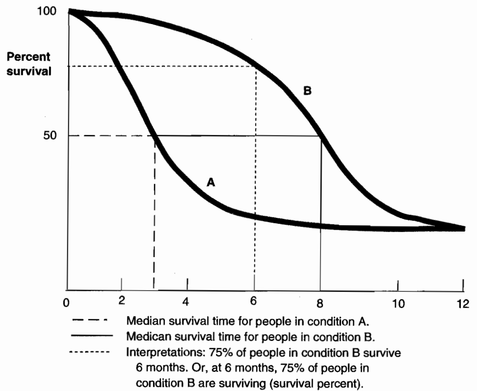
Figure 1-5. Survival Curve
